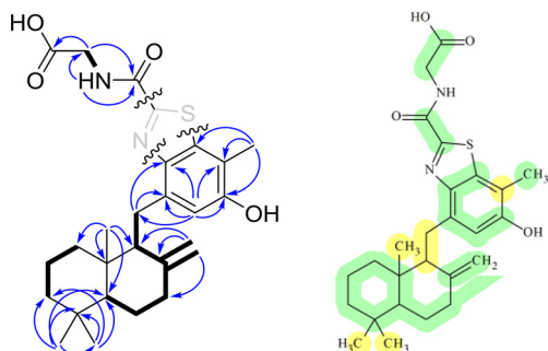
Fig. 2. The key COSY (bold) and HMBC (arrow) correlations (left) and the analysis result of the suggested feasible structure (right) of 1 by ACD/Structure Elucidator programs (colored circles on the atoms display chemical shift differences: green denotes a difference of less than 3 ppm while yellow is between 3 and 15 ppm; deviations in neural network-based algorithm: d_N(^{13}\text{C}) = 2.322 , d_N(^{13}\text{C} + ^1\text{H}) = 3.382 ).
