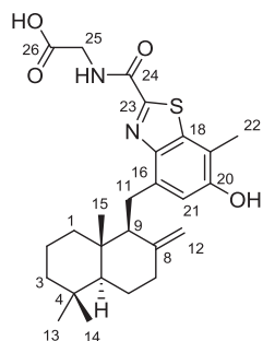
Fig. 1. Chemical structure of meroterpenothiazole A ( 1 ).
