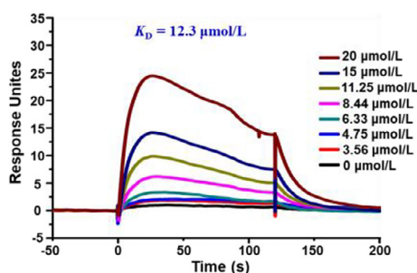
Fig. 5. The SPR result of 1 binding to RXR \alpha -LBD by Biacore T2002.4.
